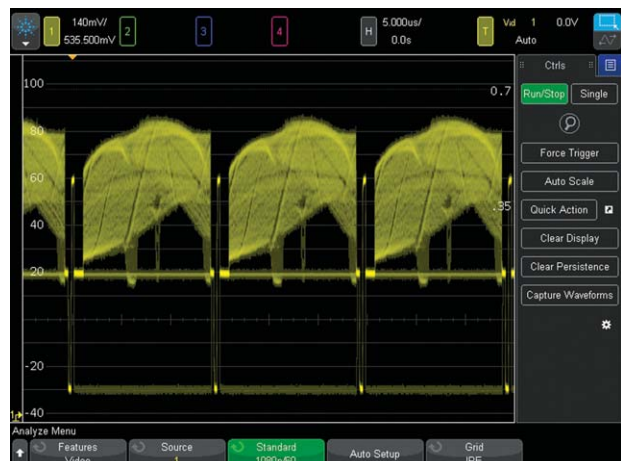
Figure 26: Triggering on 1080p HDTV signal analysis.
